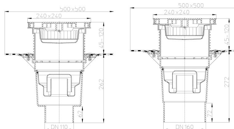
Рис. 1. HL616HLW/1 HL616HLW/5
